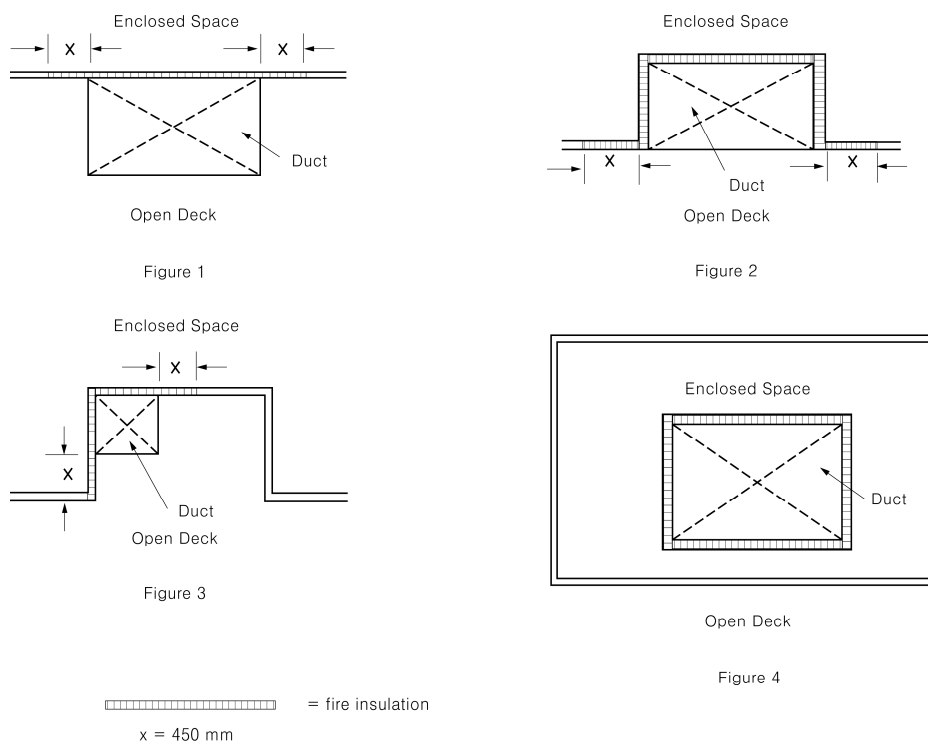
Fig 8.7.6 Examples of ducts contiguous to enclosed space
